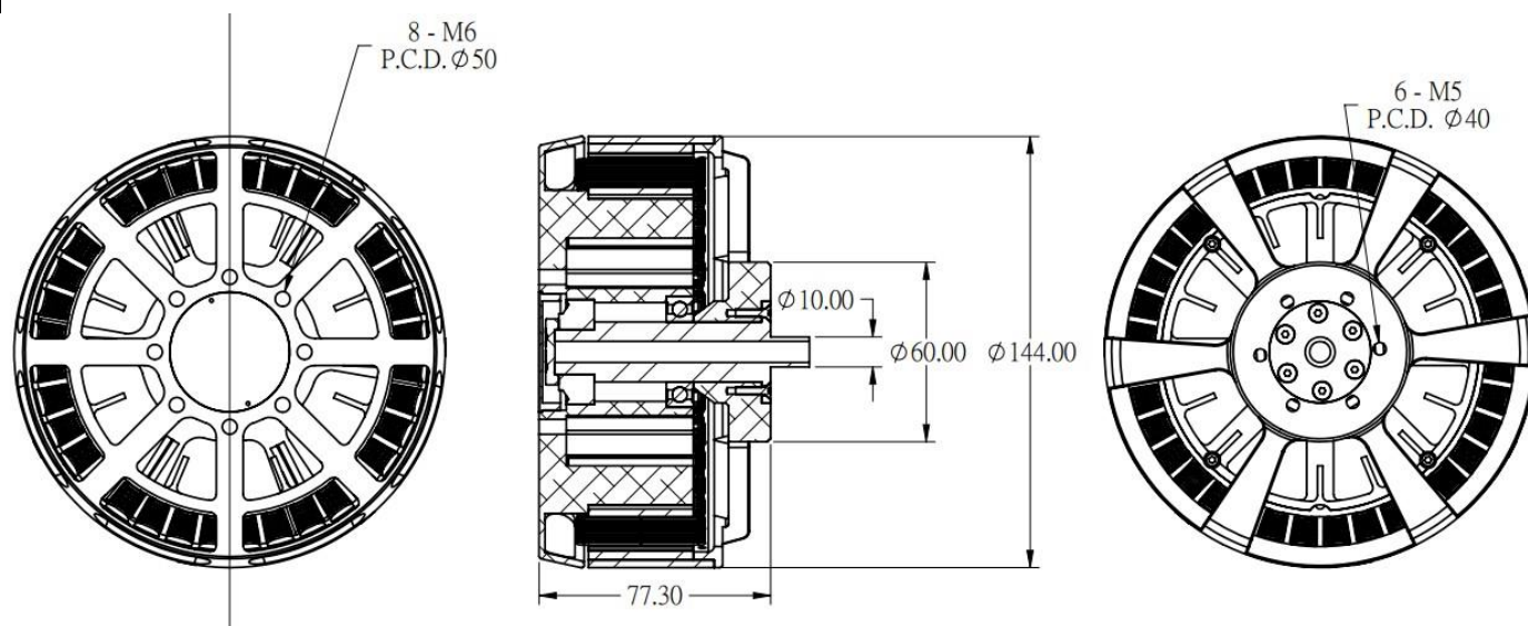
產品圖 Product Drawing
